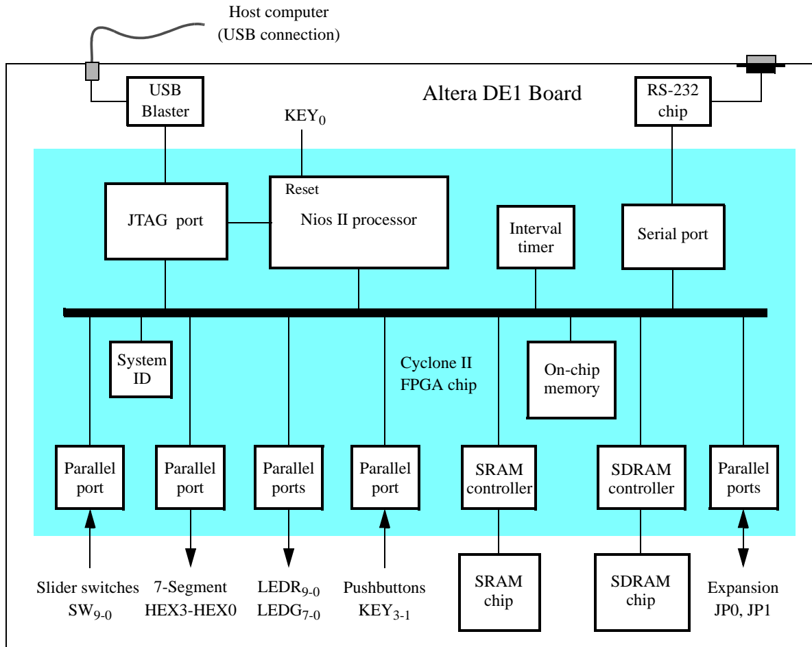
Figure 1. Block diagram of the DE2 Basic Computer.
