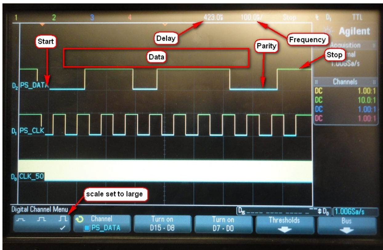
Figure 73- Zoomed in view of the data transfer
