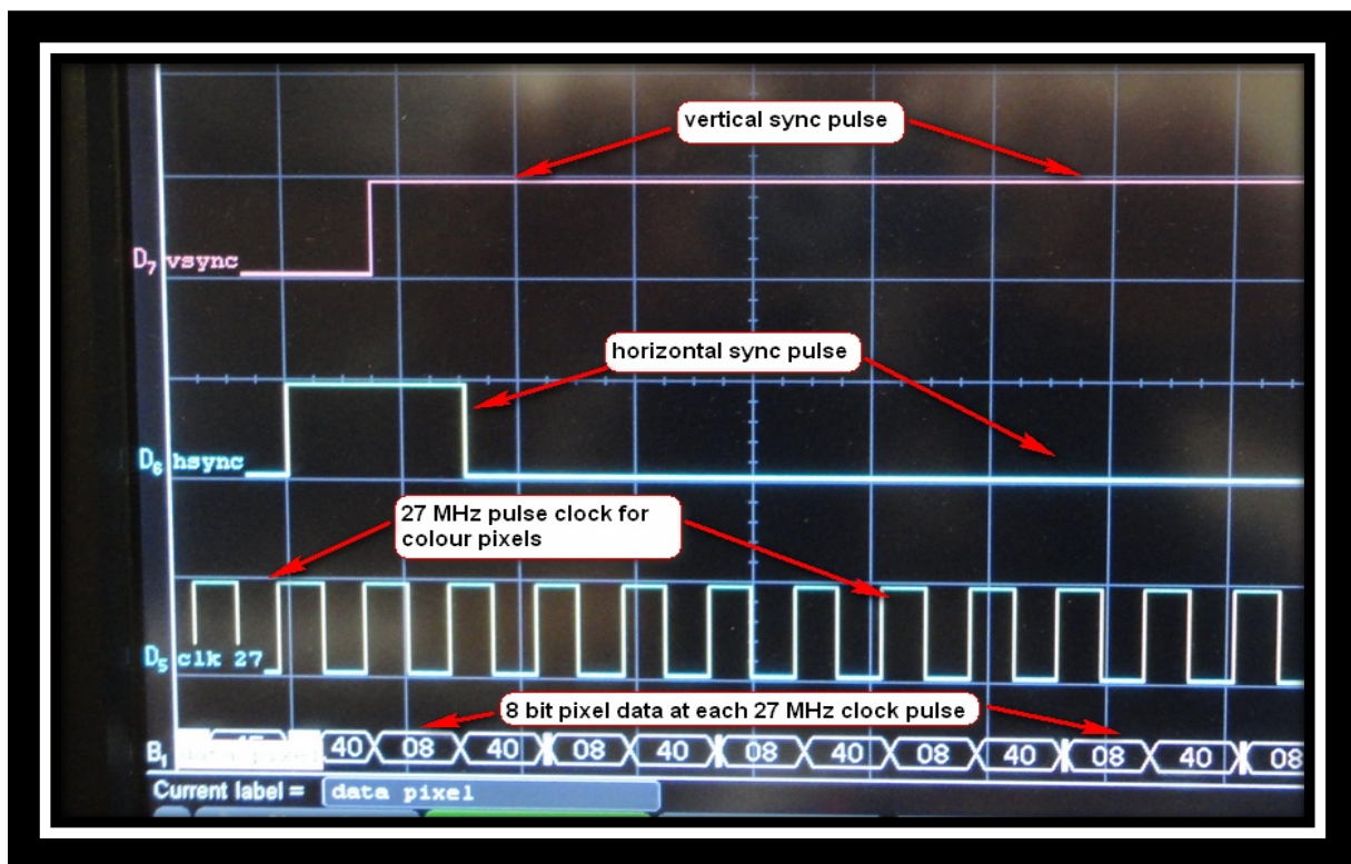
Figure 5-Zoomed in view of pixel pulses
