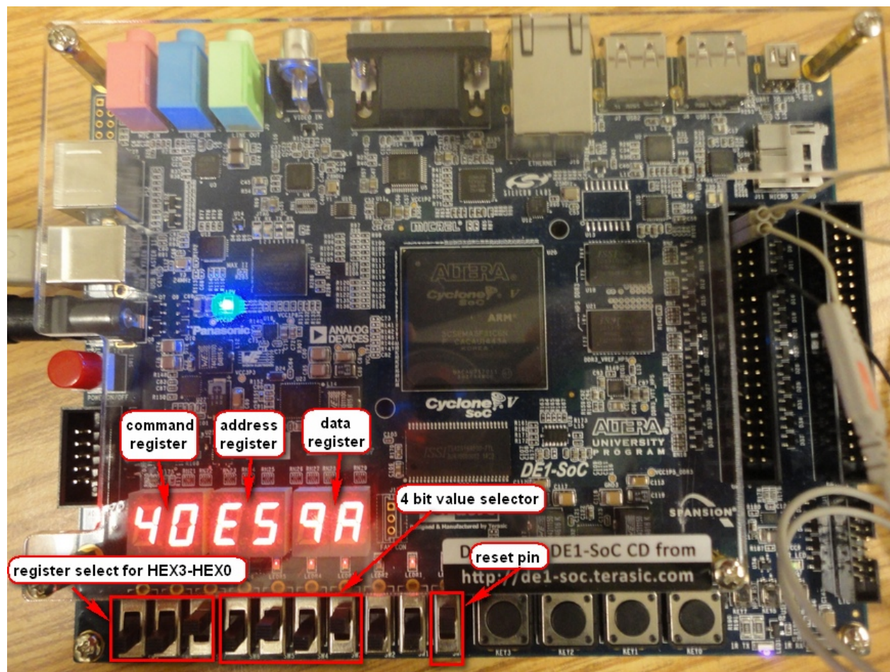
Figure 16 – HEX data values displayed on the DE1-SoC board
