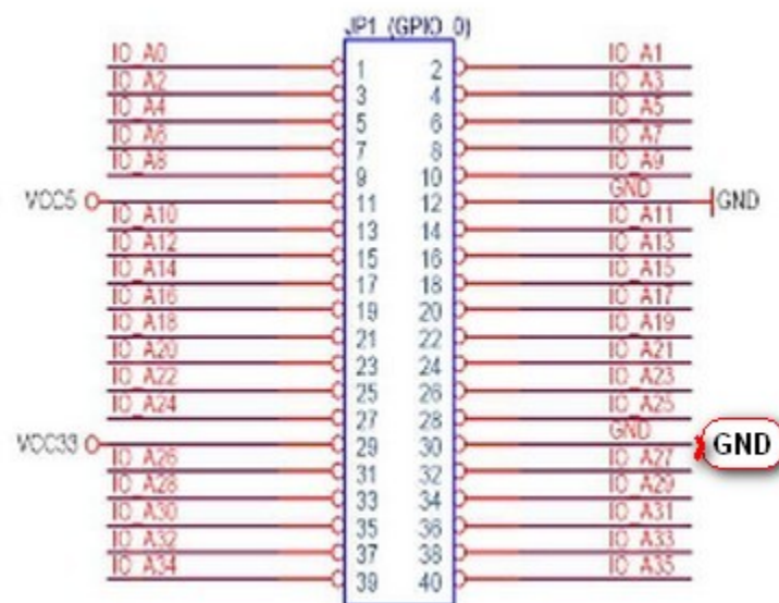
Figure 12 - Connecting digital leads to GPIO-0 on the DE1-SOC board.
