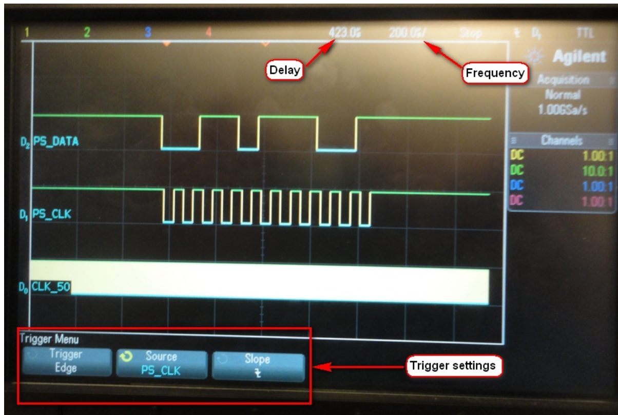
Figure 72-Sample of a data transfer from a keyboard to a device
