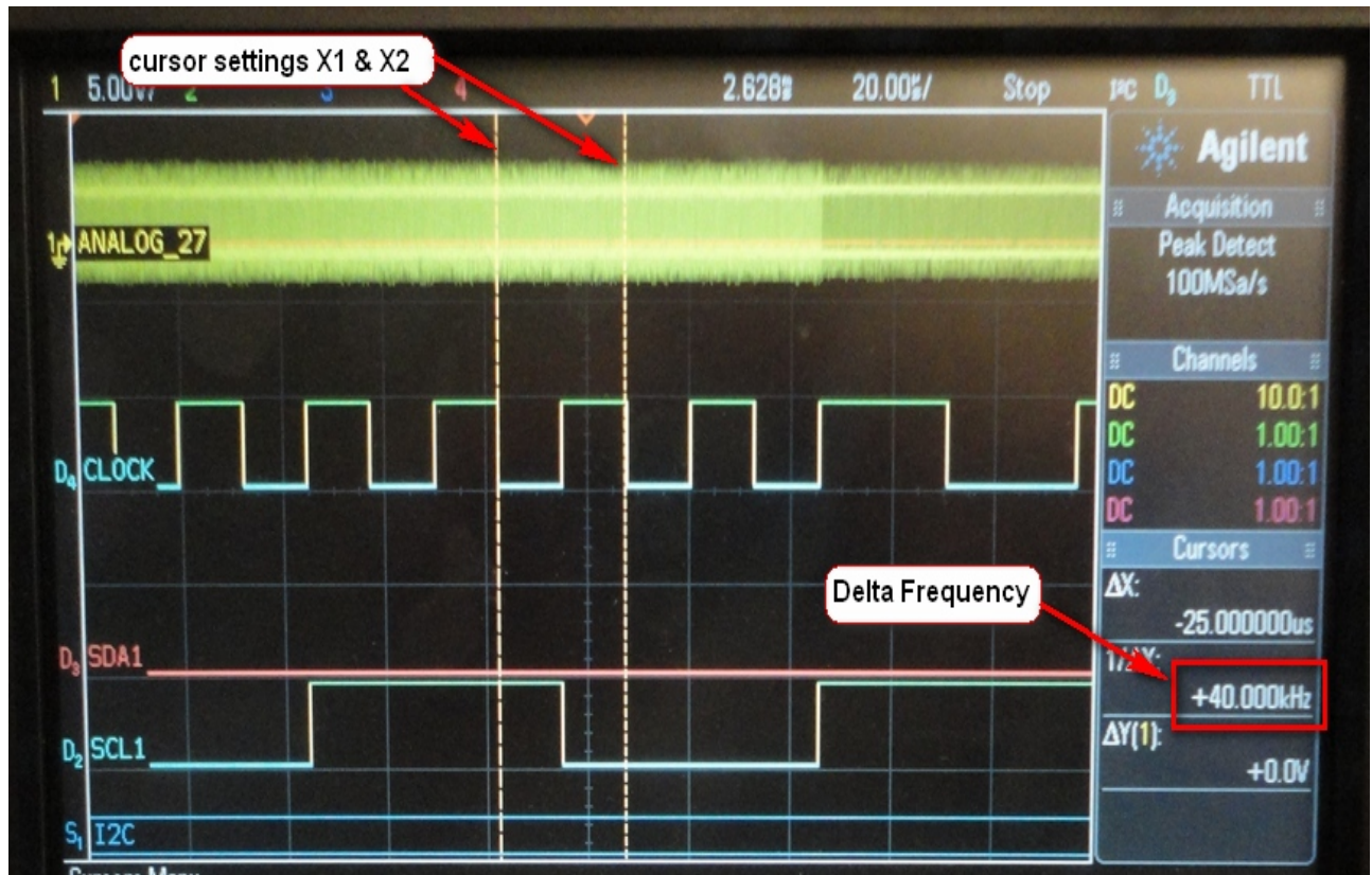
Figure 25 – The delta frequency for the default CLK_27 output
