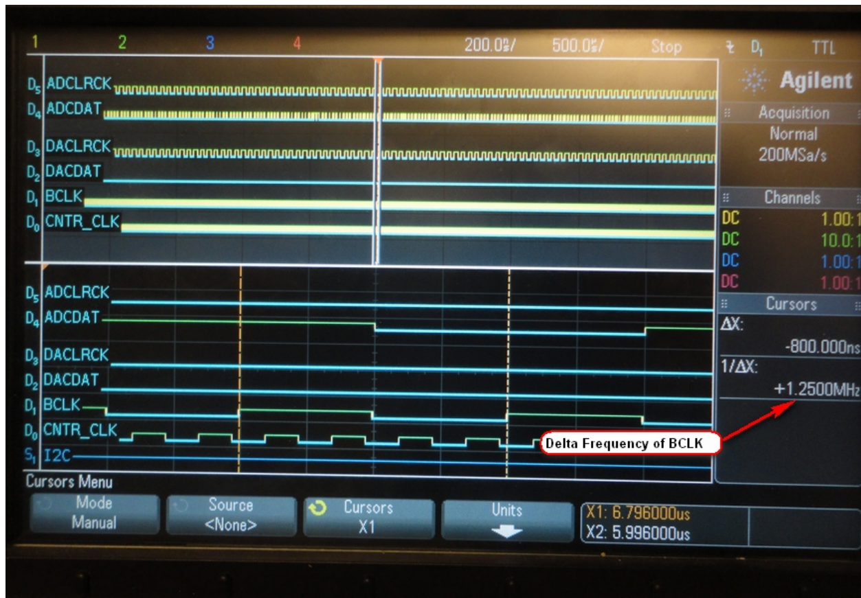
Figure 104 – Measuring the BCLK delta frequency
