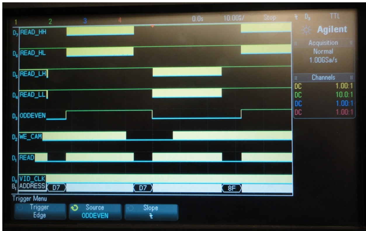
Figure 66-Sending data from the on chip memory to the monitor
