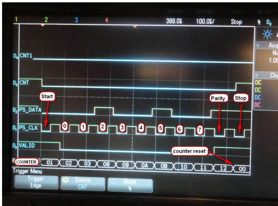
Figure 77-Trigger results for the data transfer
