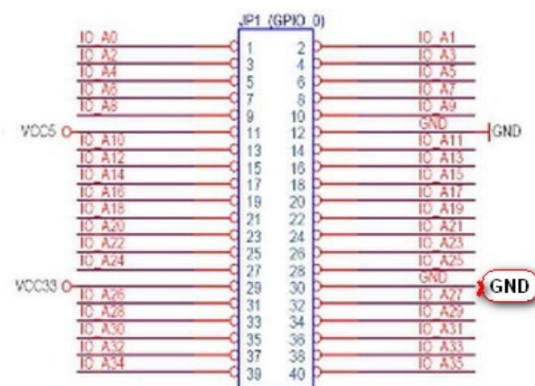
Figure 19 – Digital and analog connections to the GPIO-0 header
