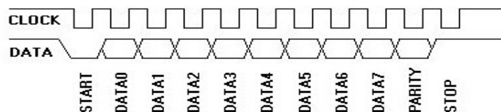
Figure 70-Timing circuit for the PS2 keyboard interface
