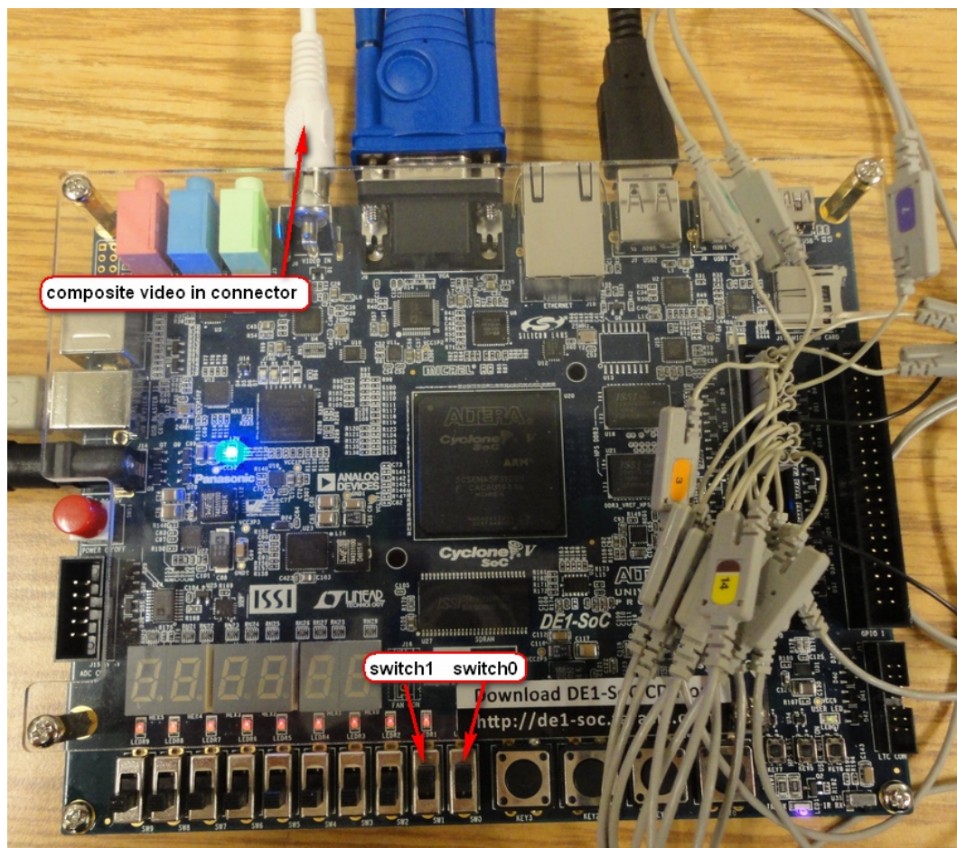
Figure 32 - Switch setting on the DE1-SOC board
