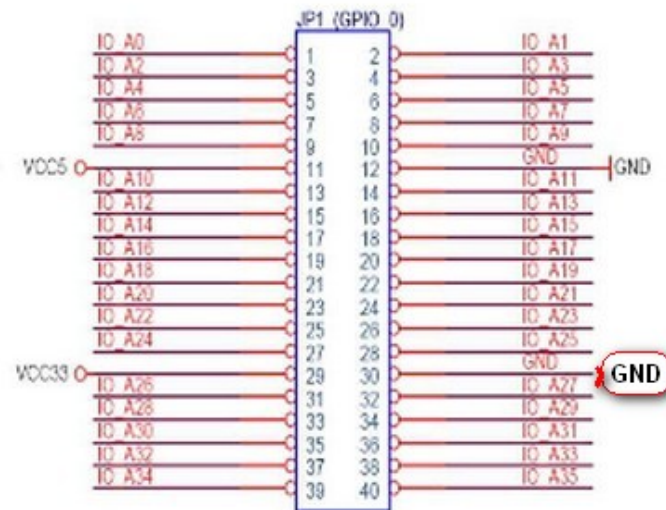
Figure 30 - Pin assignments GPIO on the Port GPIO-0
