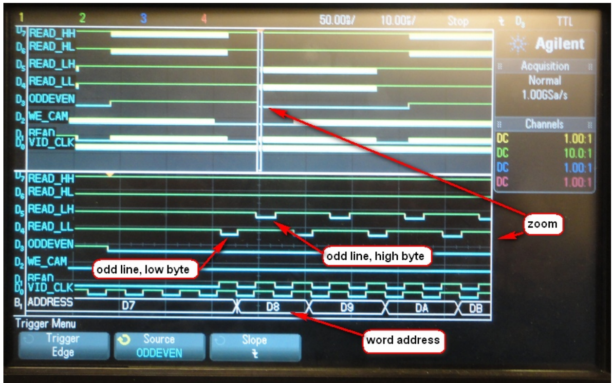
Figure 67-Zoomed in oddeven odd lines
