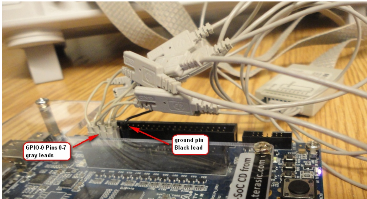
Figure 99 - Connecting the MSO-X-3024A leads from the scope to the DE1-SoC 40 pin header (GPIO-0)
