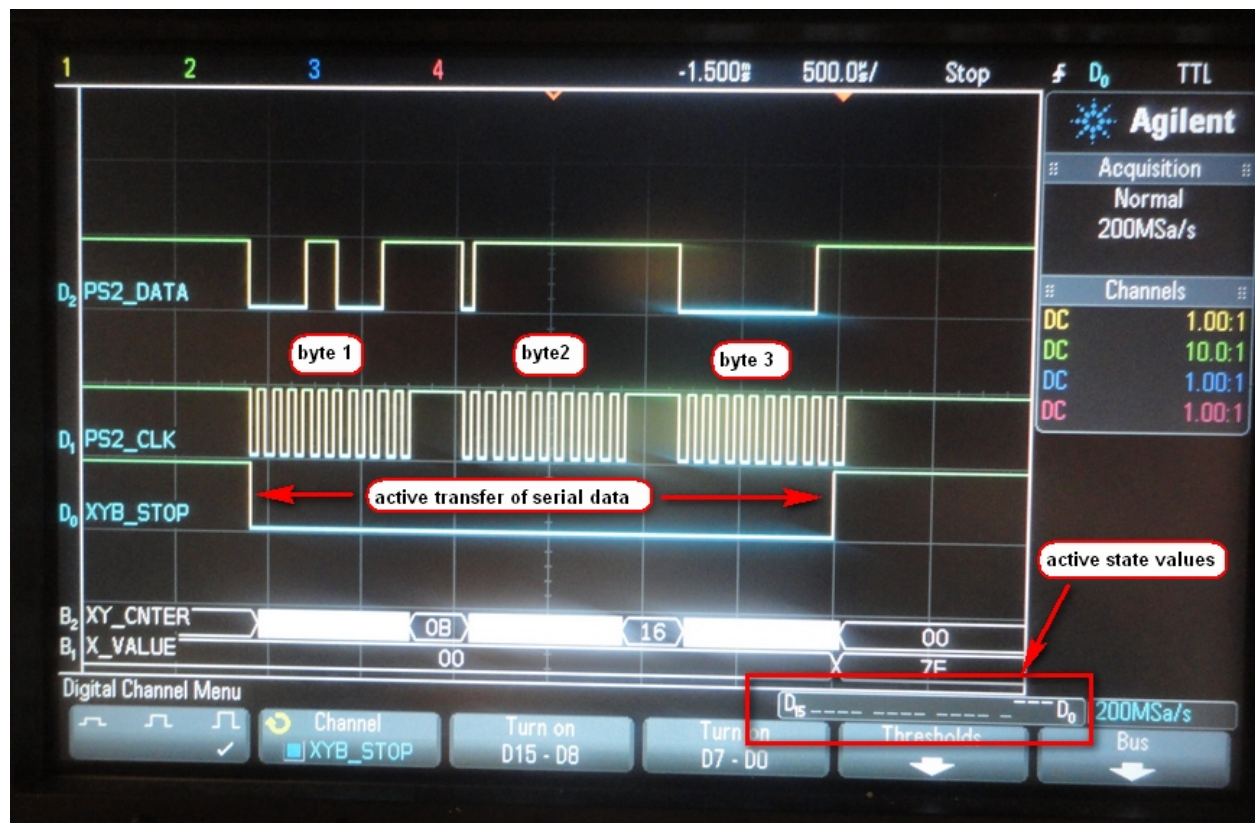
Figure 90 – The trigger event in streaming mode
