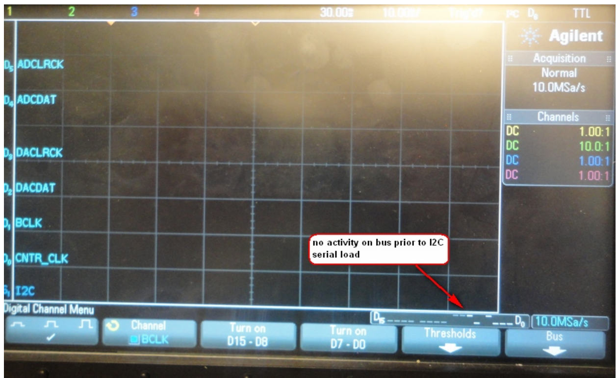
Figure 100 - No signal activity prior to the trigger event
