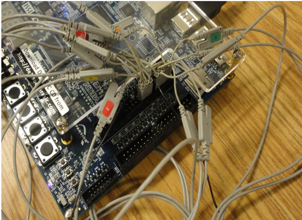
Figure 31- How to connect the digital logic probe pins from the analyzer to the DE1-SOC 40 pin header GPIO-0
