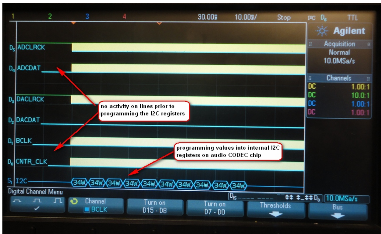
Figure 101 – Programming the internal I2C registers
