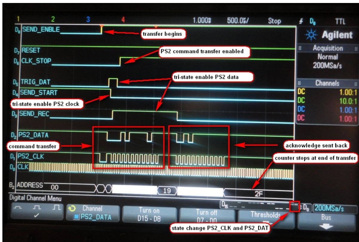
Figure 84 - Trigger command for the enabling of streaming data mode
