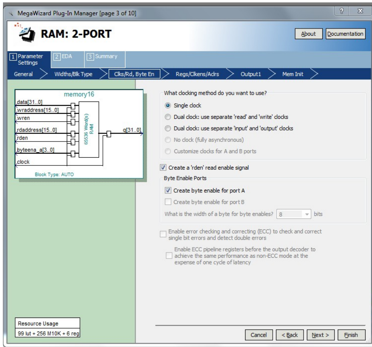
Figure 54 - Creating read enables (4 of them in this case)
