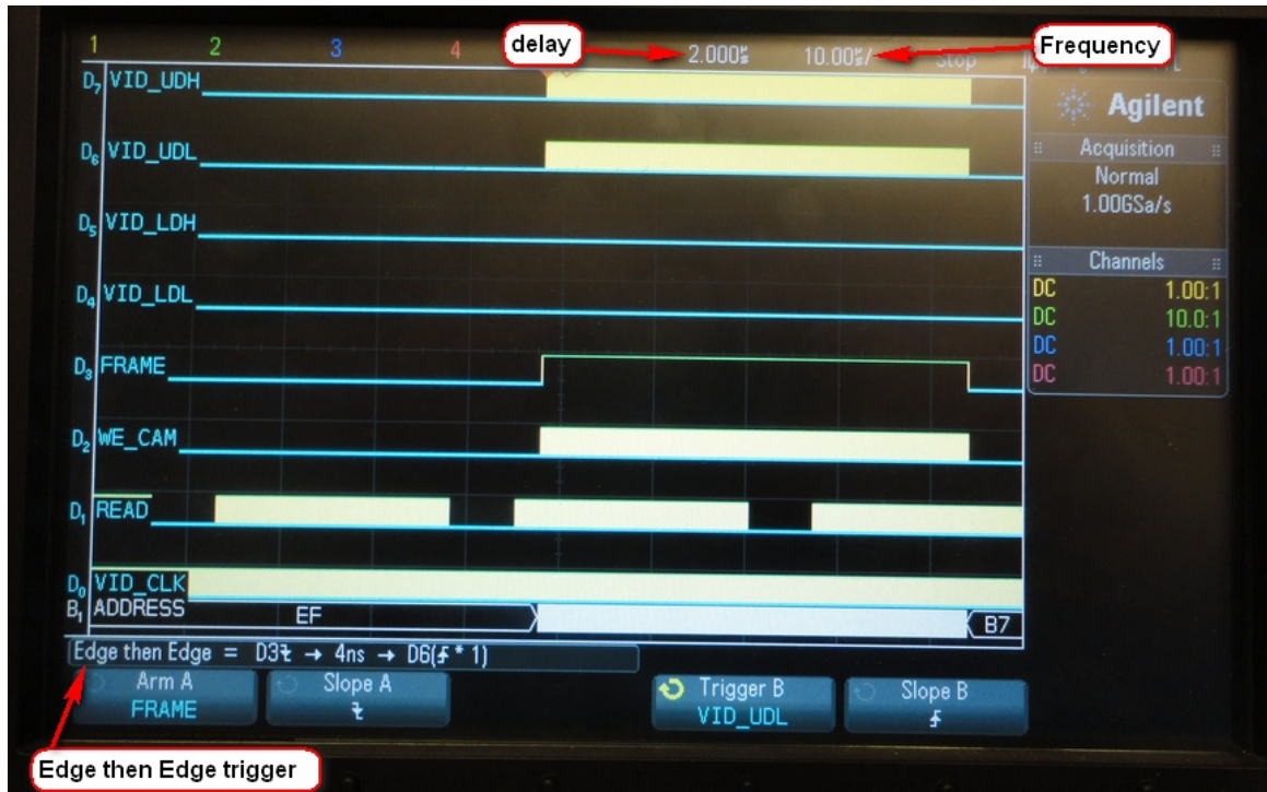
Figure 61-Even line enable from the camcorder
