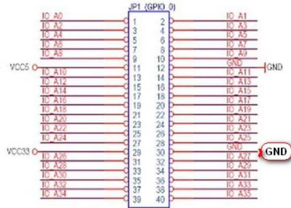
Figure 83 – Pin connections for the GPIO-0 40 pin header
