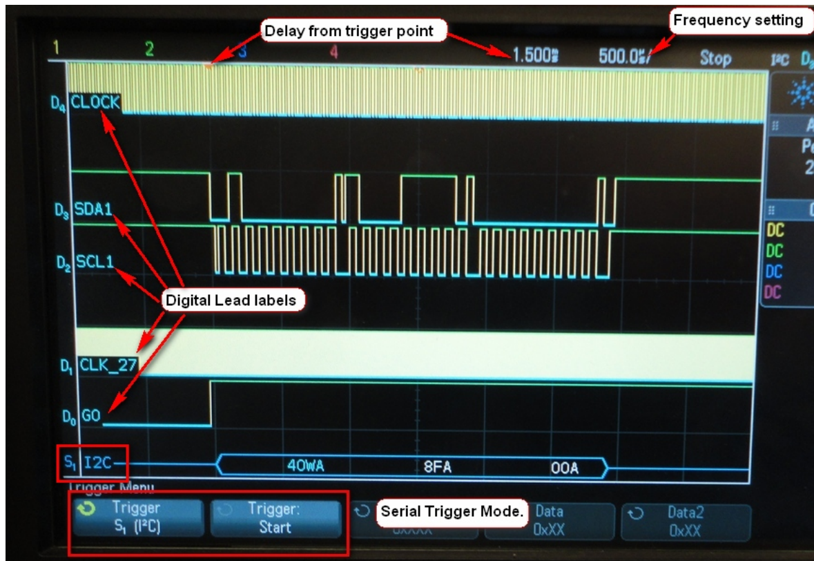
Figure 20 – The locations of the delay trigger and frequency setting
