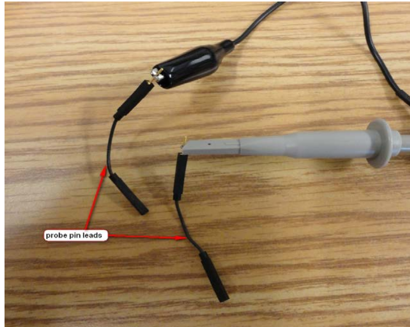
Figure 18 – Description of how to connect the probe pin leads to the analog probe
