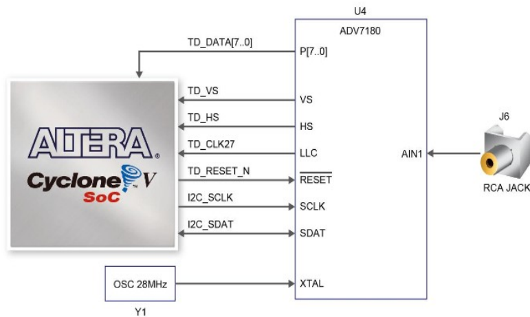
Figure 2-Block diagram of the DE1-SoC FPGA to the video decoder
