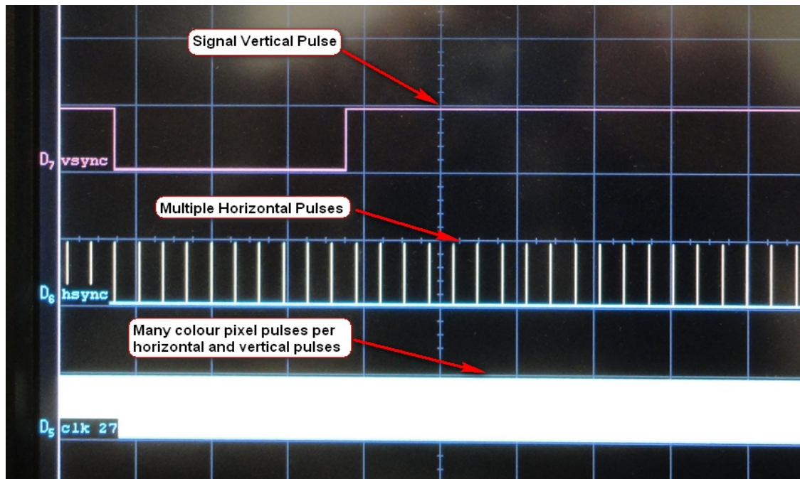
Figure 4-Zoomed in view of horizontal pulses
