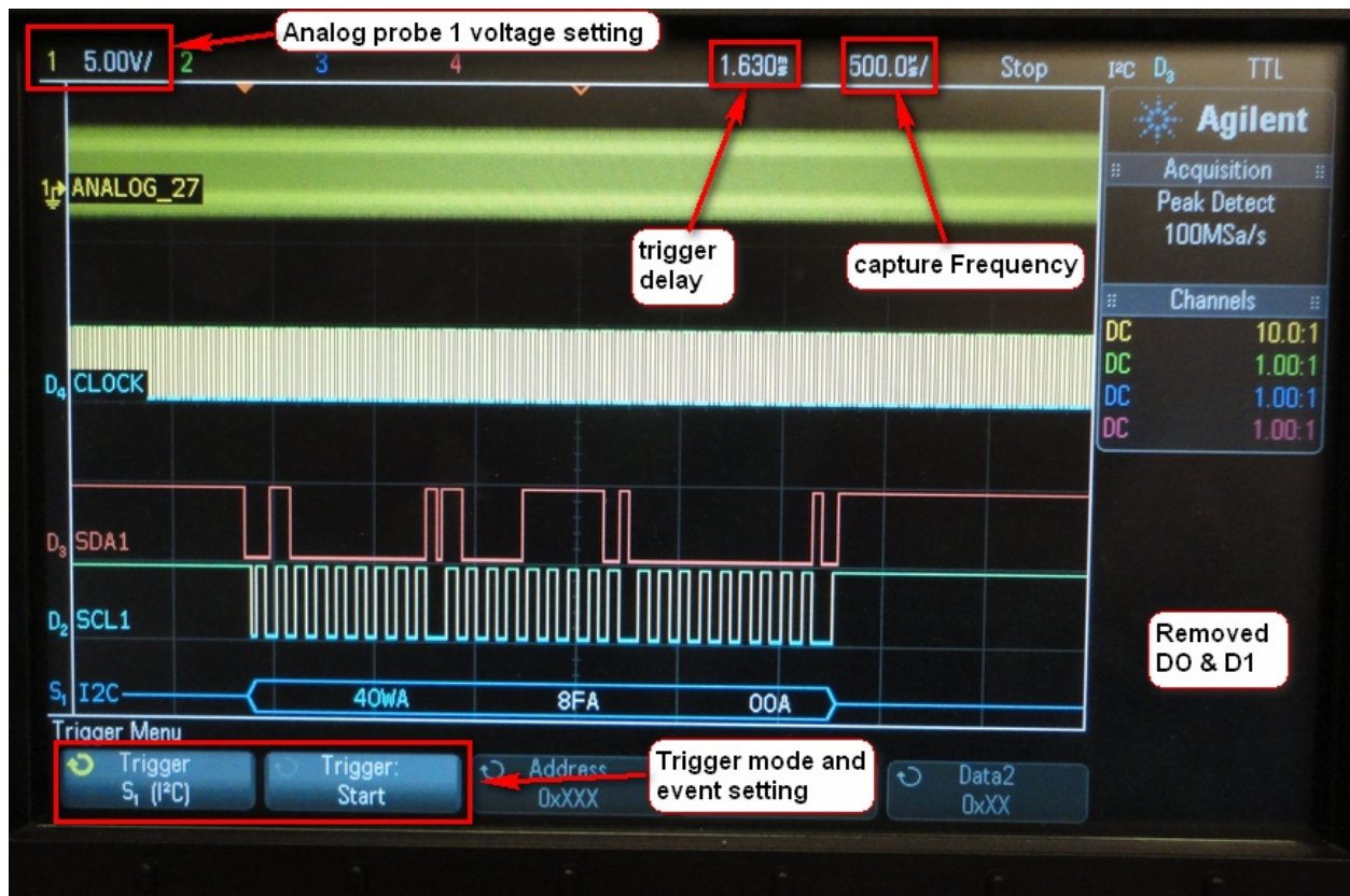
Figure 21 – Analog probe 1 input added and D0 and D1 removed.
