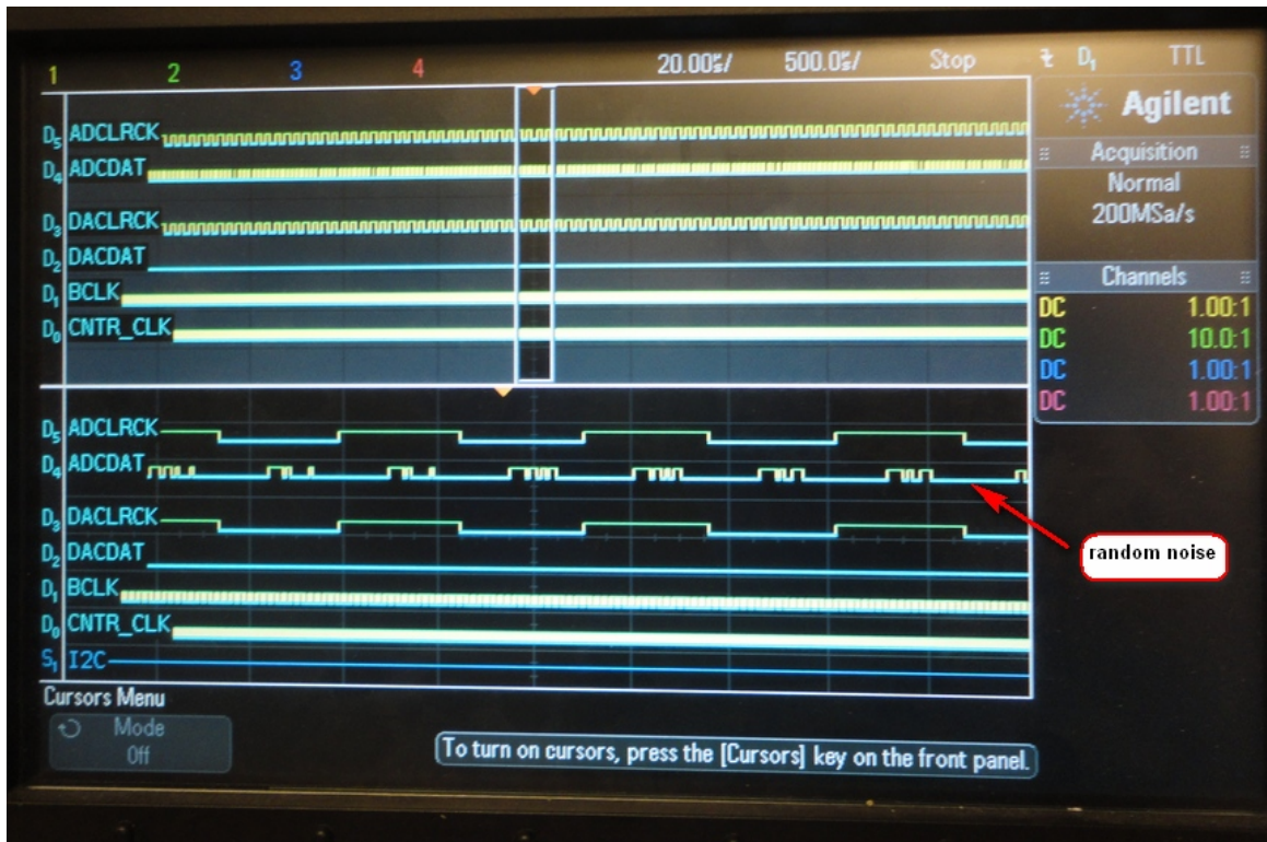
Figure 105 - Zoomed out view of the left right channel enables for the I2C format
