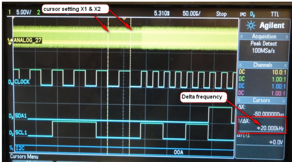
Figure 23 – Using cursors to check the delta frequency
