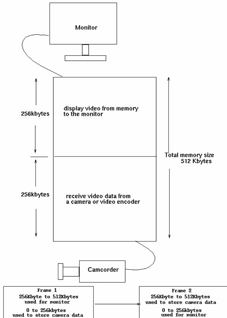
Figure 27 – Block diagram of the split memory
