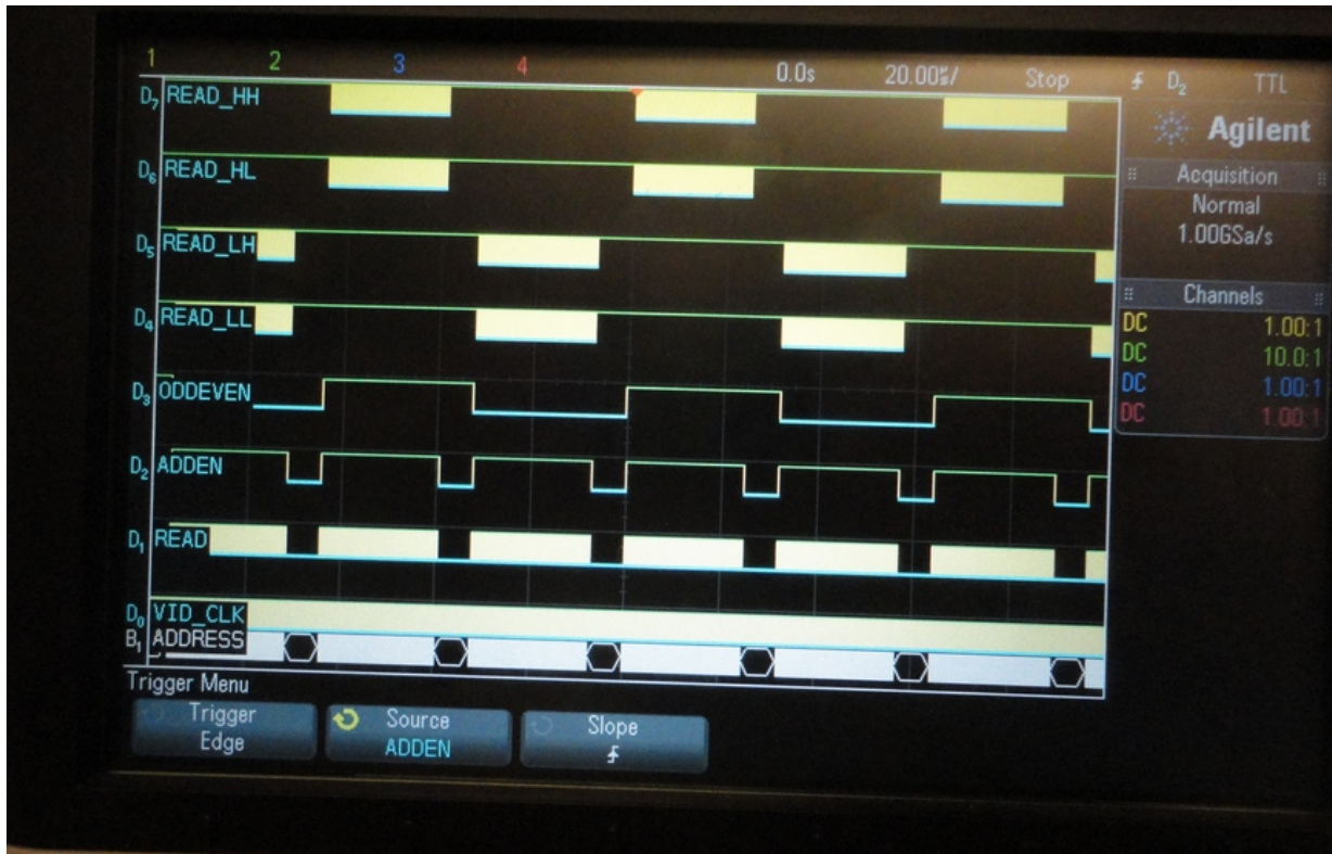
Figure 47- Address and data enable for multiple frames
