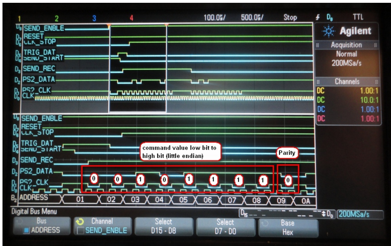
Figure 85 - Zoomed in transfer sequence
