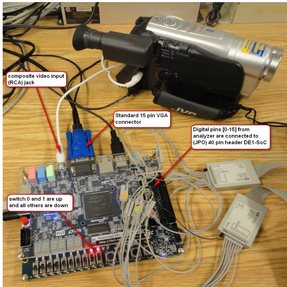
Figure 58-Layout of the video connectors
