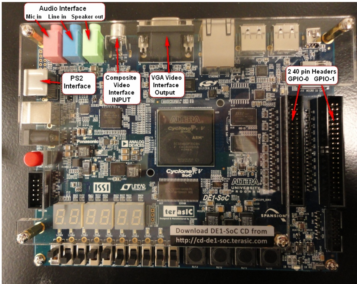
Figure 1- Location of interfaces.
